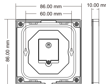
Installation diagram:
